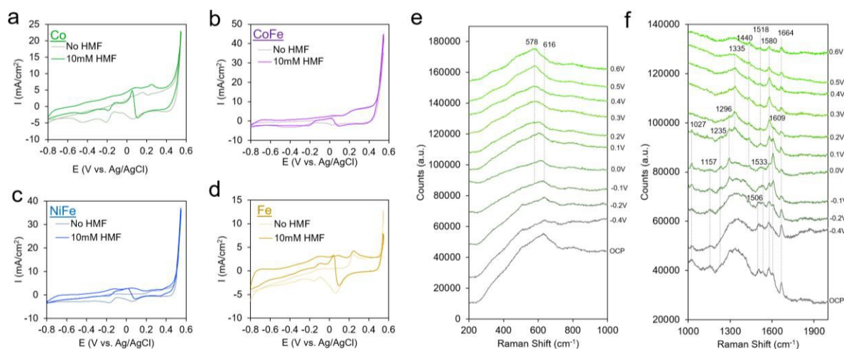
Figure 5: Extension to other transition metal thin films. Co (a), CoFe (b), NiFe (c), and Fe (d) catalysts were screened for their activity towards HMF oxidation. A closer look at AuCo catalysts with operando Raman spectroscopy in the low frequency region reveals the formation of an amorphous \text{CoO}_x surface under oxidizing conditions 35 (e), and the high-frequency region gives insight on the nature of the surface intermediates (f).
