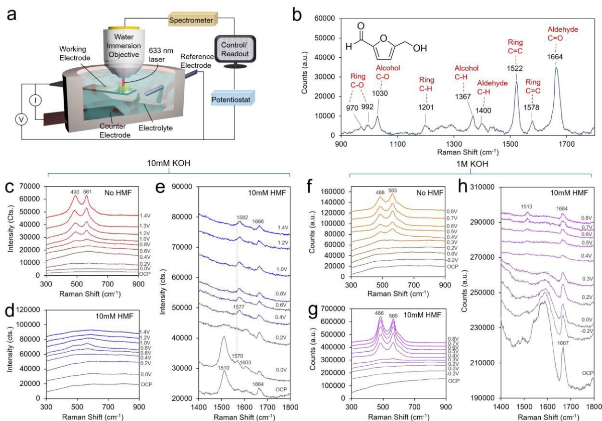
Figure 4: Operando SERS. A custom-built reaction cell and water immersion objective were employed (a). A spectrum of a 500mM aqueous solution of HMF is illustrated in (b) for reference. In 10mM KOH, NiOOH readily forms beginning at 0.6V (c) but when 10mM HMF is added to the same solution, its formation is largely suppressed, shown in the low frequency region (d). The high frequency region illustrates the HMF adsorption and reaction pathway on the surface en route to DFF (e). In 1M KOH, NiOOH for both without HMF (f) and with HMF (g) present, albeit with an altered structure. The high frequency spectra portray the surface intermediates as HMF is converted to HMFCa and to FDCA at potentials of 0.4V and above (h).
