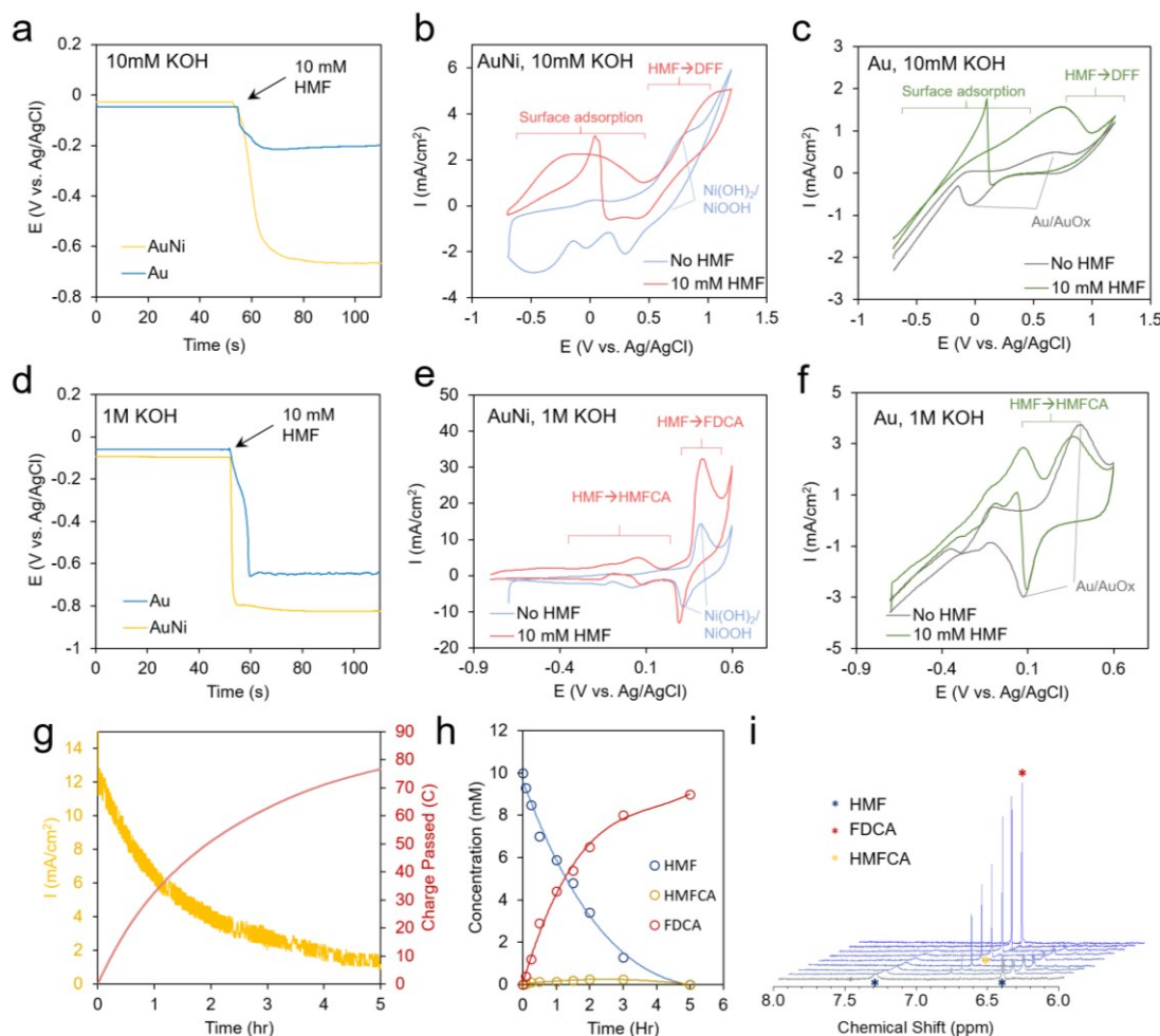
Figure 3: Electrochemical analysis. In 10 mM KOH, strong affinity of HMF to the Ni surface is evidenced by the change in open circuit potential upon injection of 10 mM HMF into the electrolyte solution (a). Enhanced current is noted from -0.6 to 0.5V AuNi (b) and from -0.2V to 1.0V for Au (c). Larger shifts in the open circuit potential are seen in 1M KOH (d) and a current enhancement is especially pronounced at 0.4V for AuNi (e) and at 0V for Au (f). A chronoamperometric scan at 0.4V shows a decreasing current as HMF is depleted (g) and converted into FDCA (h, i).
