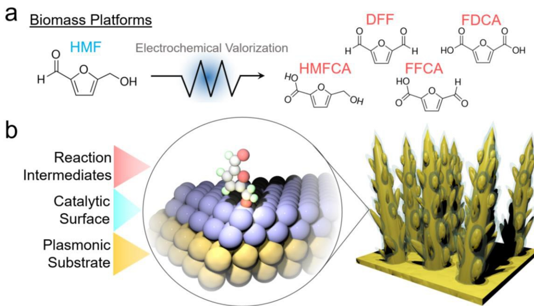
Figure 1: Possible reaction products of electrochemical oxidation of HMF (a). The designed system utilizes a plasmonic substrate for SERS enhancement to view catalyst material transformations as well as the reaction pathway on the surface (b).
