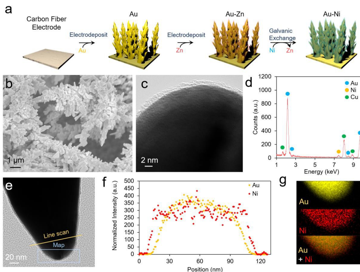
Figure 2: The AuNi catalysts are prepared through a facile electrodeposition and galvanic exchange method (a). The resultant materials are high surface area Au dendrites (b) with a 1-2 nm shell of amorphous Ni (c). EDS analysis only shows peaks stemming from Au, Ni and Cu, the latter originating from the Cu TEM grid employed in this work (d). A catalyst tip (e) was further evaluated with an EDS linescan (f) and elemental map (g) to show the conformal nature of the Ni layer.
