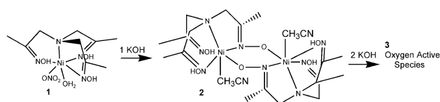
Fig. 1 Formation of the oxygen active species, 3 .
