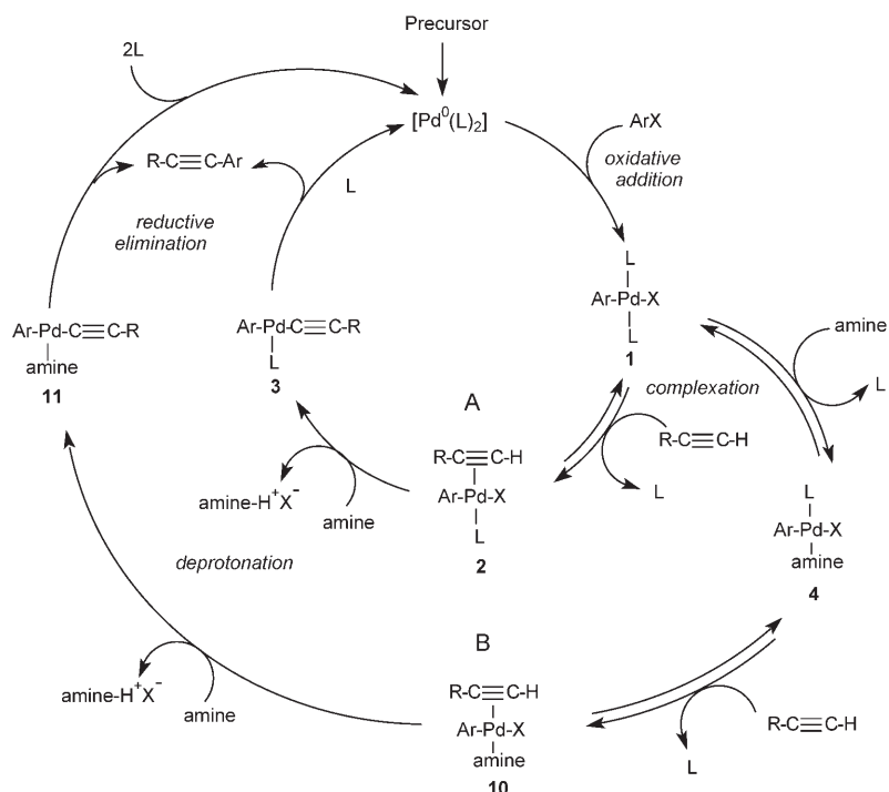
Scheme 5. Mechanism of the copper-free palladium-catalyzed Sonogashira reaction ( \text{R} = \text{CH}_2\text{-CH}_2\text{-OH} ). Path A : the amine is a less good ligand than the alkyne for the \text{Pd}^{\text{II}} center in [\text{PdX}(\text{Ar})(\text{L})_2] ( \text{L} = \text{PPh}_3 with amine = piperidine or morpholine). Path B : the amine is a better ligand than the alkyne for the \text{Pd}^{\text{II}} center in [\text{PdX}(\text{Ar})(\text{L})_2] ( \text{L} = \text{AsPh}_3 , amine = piperidine).
