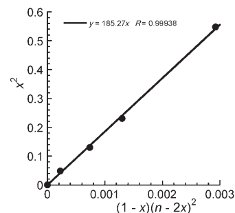
Figure 2. Determination of the equilibrium constant K' for the reaction between complex 7b and 4bm formed after addition of morpholine ( n equiv) to complex 7b ( C_0 = 6.67 \text{ mM} ) in CDCl 3 at 25 °C. K'' = [\mathbf{4bm}]^2/([\text{R}_2\text{NH}]^2[\mathbf{7b}]) = 4x^2/[C_0(1-x)(n-2x)^2] ( x = molar fraction of 4bm ). Plot of x^2 versus (1-x)(n-2x)^2 . The slope of the straight line gave K'' = 110\,900 \text{ M}^{-1} . K' = K''^{1/2} = 333 \text{ M}^{-1/2} (Scheme 3).
