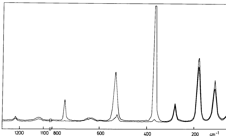
Fig. 2. Raman spectrum of I: 1 mm o.d. capillary, slit width 4 \text{cm}^{-1} , parallel and perpendicular polarization.
