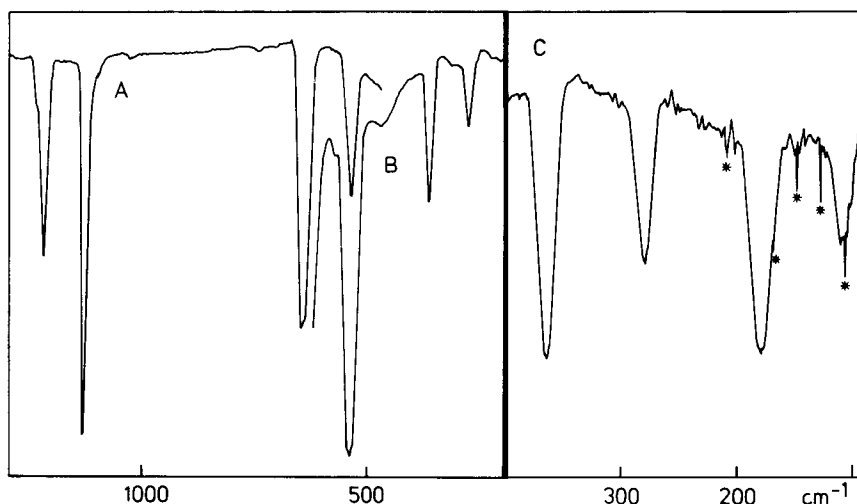
Fig. 1. IR spectrum of I: A: 10 cm cell, KBr windows, 3 mbar, resolution 1–2 \text{cm}^{-1} . B: 18 cm cell, polythene windows, 12 mbar, resolution 2–4 \text{cm}^{-1} . C: 18 cm cell, polythene windows, 30 mbar, resolution 1 \text{cm}^{-1} . Rotational lines of HCl are marked by an asterisk.
