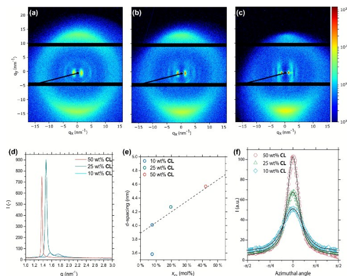
Figure 2 Structural characterization of the pristine polymer films. (a-c) 2D x-ray diffractograms of LCNs containing 10, 25, and 50 wt% CL , respectively. N.B. The visible asymmetry and dark region is caused by the partial blocking of the scattered x-rays by the sample holder. (d) Azimuthal integration of the small angle region of the x-ray diffractograms obtained from MAXS measurements. (e) d -spacing as a function of x_{\text{CL}} . (f) Radial integration of the wide angle signal ( q \approx 14 nm -1 ).
