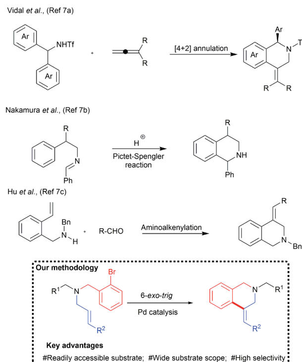
Chart 1 Methods for the synthesis of C4-substituted tetrahydroisoquinolines and our methodology.
