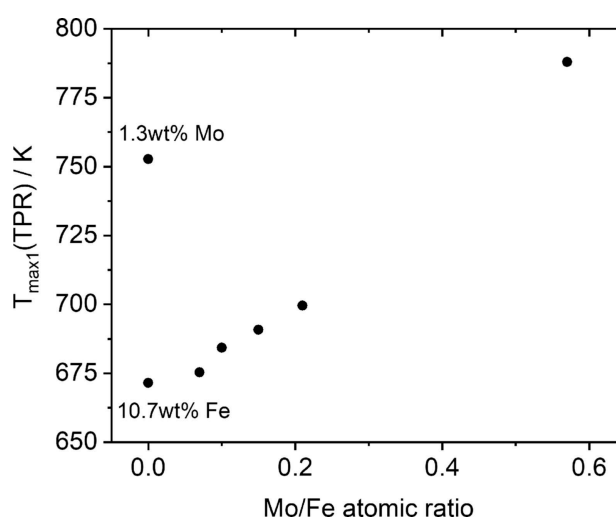
Figure 7. Temperature of the first TPR maxima, T_{\text{max1}}(\text{TPR}) , as function of Mo/Fe atomic ratio. Samples 1.3 wt% \text{Mo\_SBA-15} and 10.7 wt% \text{Fe\_SBA-15} are depicted at Mo/Fe atomic ratio of 0. TPR experiments were performed in 5% \text{H}_2 in argon at a heating rate of 10 K/min.
