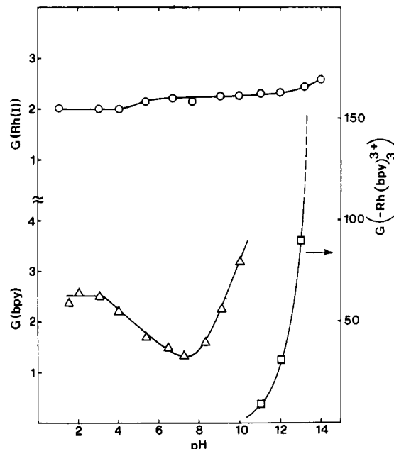
Figure 10. G(\text{bpy}) , G(\text{Rh(I)}) , and G(-\text{Rh}(\text{bpy})_3^{3+}) as a function of pH from the continuous radiolysis of deaerated \text{Rh}(\text{bpy})_3\text{Cl}_3 (150 \mu\text{M} ) solution containing 0.1 M 2-propanol. Conditions are the same as for Figure 8 except for the determination of G(-\text{Rh}(\text{bpy})_3^{3+}) where the radiation dose was 6.10 \times 10^{19} \text{eV L}^{-1} (0.98 krd) and the optical path was 2 mm.
