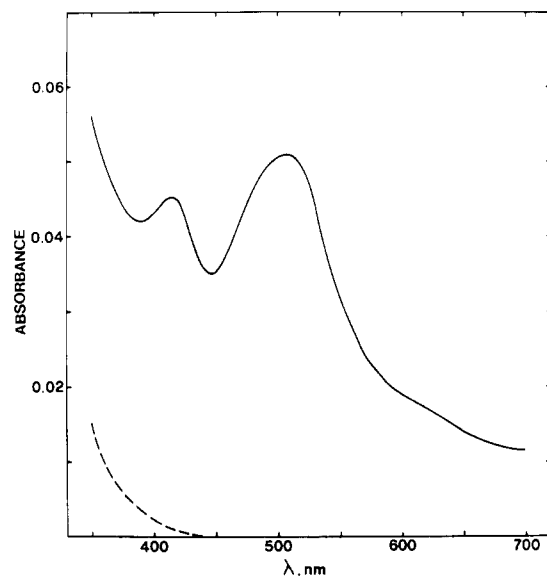
Figure 9. Visible spectral changes observed from the continuous radiolysis of deaerated \text{Rh}(\text{bpy})_3\text{Cl}_3 (150 \mu\text{M} ) solution containing 0.1 M 2-propanol and 10% buffer solution at an initial pH of 7.2. Optical path length = 2 mm; dose = 2.78 \times 10^{21} \text{eV L}^{-1} (44.5 krd). After radiolysis, —; after addition of \text{O}_2 , ----.
