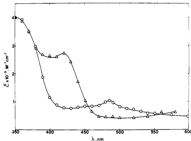
Figure 2. Spectra of pulse radiolysis transients. (O) Visible spectrum of \text{Rh}(\text{bpy})_3^{2+} measured \sim 80 \mu\text{s} after the pulse; optical path length = 2 cm, dose/pulse = 1.5 krd. The following conditions were used: (a) 50 \mu\text{M} \text{Rh}(\text{bpy})_3^{3+} , 0.5 M 2-propanol, Ar-purged solution, natural pH; (b) same but at pH 3; (c) same but at pH 10; (d) 50 \mu\text{M} \text{Rh}(\text{bpy})_3^{3+} , 0.5 M 2-propanol, 0.1 M acetone, Ar-purged solution, natural pH. In evaluating \epsilon , G(\text{Rh}(\text{bpy})_3^{2+}) = 6.0 was assumed. ( \Delta ) Visible spectrum of product of reaction of H atoms and \text{Rh}(\text{bpy})_3^{3+} at pH 1 in the presence of 0.5 M tert -butyl alcohol measured \sim 80 \mu\text{s} after the pulse; optical path length = 2 cm, dose/pulse = 1.5 krd; Ar-purged solutions. The observed spectrum was corrected for incomplete scavenging of H and for the decay of the transient. In evaluating \epsilon , G(\text{transient}) = 3.3 was assumed.
