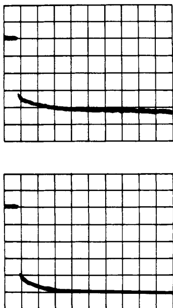
Figure 11. CRO traces relating to the ring-opening equilibrium of \text{Rh}(\text{bpy})_3^{2+} . Solutions contain 540 \mu\text{M} \text{Rh}(\text{bpy})_3^{3+} , 0.5 \text{ M} 2-propanol, 0.1 \text{ M} acetone at \text{pH } 10 . Optical path length = 2 \text{ cm} ; wavelength of observation = 485 \text{ nm} . Upper trace: abscissa = 200 \mu\text{s}/\text{div} , ordinate = 1.03\% \text{ abs}/\text{div} , dose/pulse = 1.4 \text{ krd} . Lower trace: abscissa = 100 \mu\text{s}/\text{div} , ordinate = 2.60\% \text{ abs}/\text{div} , dose/pulse = 4.2 \text{ krd} .
