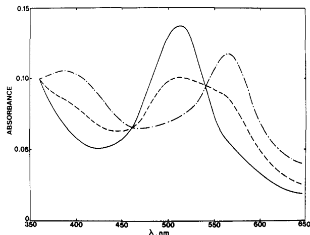
Figure 4. Visible spectra from the single pulse experiment: [\text{Rh}(\text{bpy})_3(\text{ClO}_4)_3] = 230 \mu\text{M} , 0.1 M 2-propanol, Ar-purged solution, pH 10, optical path length = 1 cm, dose/pulse = 6.5 krd. Spectra determined at 2 min (—), 5 min (---), and 20 min (-.-) after the pulse. Upon standing beyond 20 min, the clear solution became turbid and a precipitate formed. Assuming \epsilon_{510} = 9500 \text{ M}^{-1} \text{ cm}^{-1} for the initially absorbing species, \epsilon_{565} \geq 8400 \text{ M}^{-1} \text{ cm}^{-1} for the violet species.
