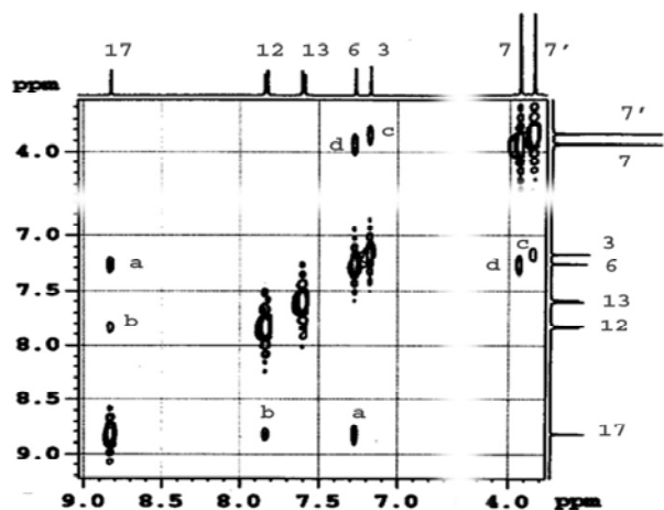
Figure 1. NOESY spectrum of compound 9.
