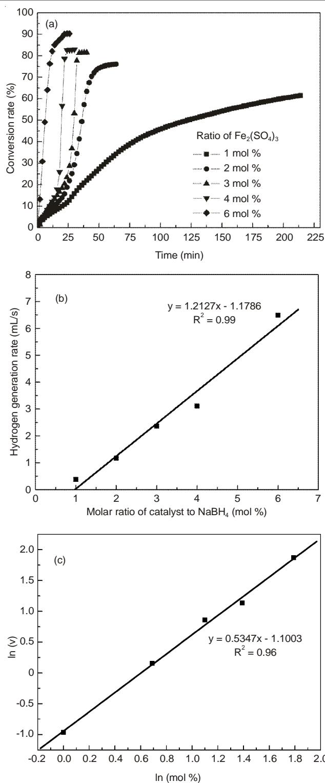
Fig. 5. (a) Hydrogen generation evolution; (b) Effect of mixture ratio of catalyst on hydrogen generation rate ( v ); (c) H 2 -generated flow rate versus mixture ratio of Fe 2 (SO 4 ) 3 both in logarithmic scale. (2 g NaBH 4 , feed water flow rate of 0.20 mL/min, at 19 °C)
