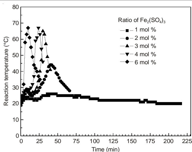
Fig. 3. Reaction temperature as a function of time under 2 g \text{NaBH}_4 , feed water flow rate of 0.20 mL/min, initial temperature of 19^\circ\text{C}
