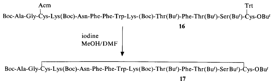
Scheme 7. Formation of the disulfide ring in the protected 1–14 somatostatin derivative 16
