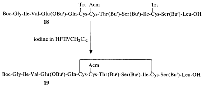
Scheme 8. Selective formation of the disulfide ring A6–A11 in the protected A(1–13) segment 18 of human insulin
