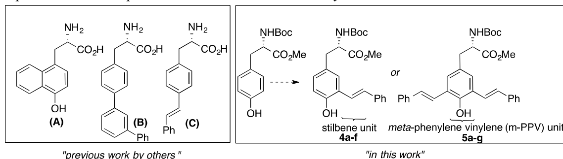
Figure 1. Fluorescent UAAs derived from tyrosine/phenylalanine by extending the \pi -conjugation of aromatic side chain.
