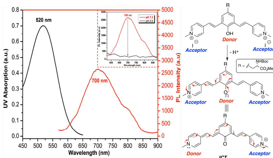
Figure 6. Absorption and emission spectra (left) of NIR emission of deprotonated 5g ; c = 100 \mu\text{M} dissolved in HEPES buffer (pH 7.3). Shown in inset is quenching of NIR emission upon acidification (pH 2) due to the protonation of phenolate; a schematic representation (right) showing the origin of NIR emission through ICT mechanism
