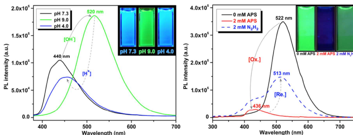
Figure 5. pH (left) and redox (right) sensitivity of compound 5b . Emission spectra were recorded using 50 \mu M and 10 \mu M solutions, respectively
