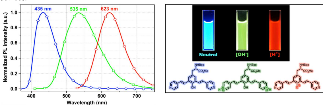
Figure 4. Emission spectra of 5f in neutral (blue), acidic (green) and basic (red) environment showing the RGB emission
