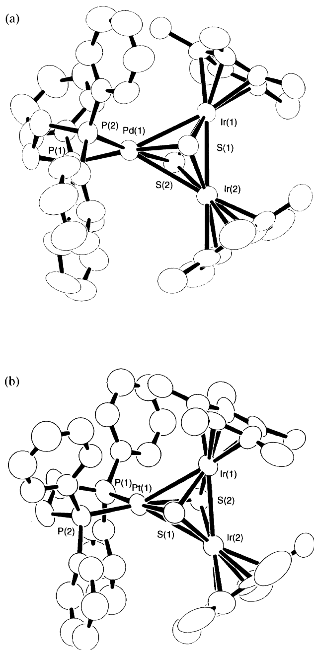
Fig. 2. Structures of the cationic parts in 9\text{-CH}_3\text{COCH}_3 (a) and 10\text{-CH}_3\text{COCH}_3 (b). Hydrogen atoms are omitted for clarity. Thermal ellipsoids are shown at the 50% probability level.
