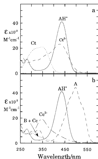
Figure 1. Absorption spectra of the species derived from 4'-hydroxyflavylium ion in aqueous solution at 25 °C: a) \text{AH}^+ , \text{Ct} , and \text{Ct}^{2-} ; b) \text{A} , \text{AH}^+ , \text{Cc}^{2-} , and \text{B} and \text{Cc} mixture at pH = 7.
