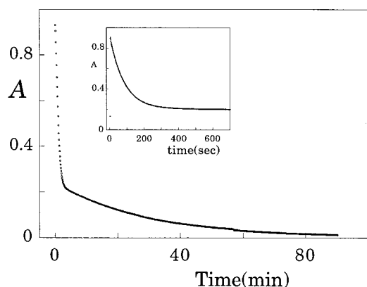
Figure 2. Decay of the absorbance at 500 nm after a pH jump of 4'-hydroxyflavylium ( \text{AH}^+ ) from pH = 1 to pH = 7 in aqueous solution at 55 °C. The inset shows the first part of the decay for a solution at 25 °C.
