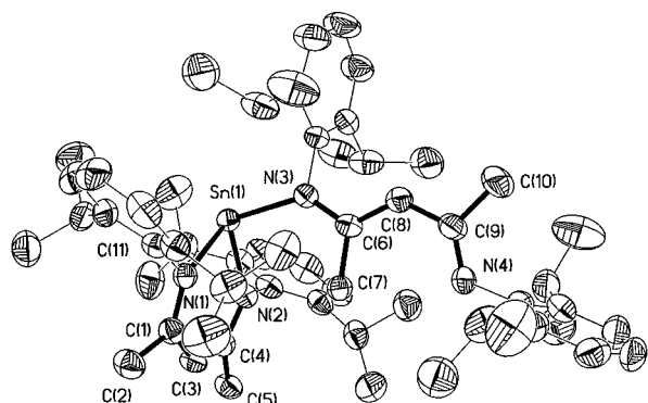
Figure 4. Thermal ellipsoid plot (50%) of 7 . H atoms are not shown. Important structural data are given in Table 1.
