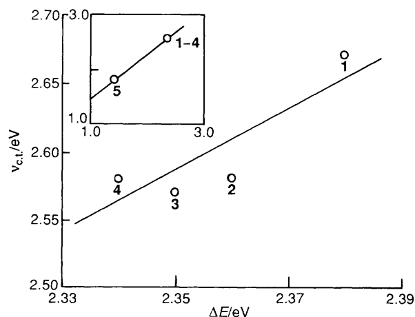
Fig. 4 Linear correlation between \nu_{\text{c.t.}} and \Delta E_{\text{ox/red}} for [\text{RuL}^2(\text{bipy})_2][\text{ClO}_4]_2 \cdot \text{H}_2\text{O} 1, [\text{RuL}^1_3][\text{ClO}_4]_2 \cdot \text{H}_2\text{O} 2, [\text{RuL}^2_2(\text{bipy})][\text{ClO}_4]_2 \cdot \text{H}_2\text{O} 3, [\text{RuL}^2_3][\text{ClO}_4]_2 \cdot \text{H}_2\text{O} 4 and cis - [\text{RuCl}_2\text{L}_2] 5
