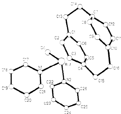
Fig. 1. View of the structure of one of the [\text{Ru}(\eta^6\text{-C}_{16}\text{H}_{16})\text{Cl}(\text{C}_5\text{H}_5\text{N})_2]^+ cations showing the atom labelling scheme. Important parameters: \text{Ru}(1)\text{--Cl}(1) 2.404(6), \text{Ru}(1)\text{--N}(1) 2.166(16), \text{Ru}(1)\text{--N}(2) 2.133(20), \text{Ru}(1)\text{--C}(1) 2.365(21), \text{Ru}(1)\text{--C}(2) 2.248(22), \text{Ru}(1)\text{--C}(3) 2.161(21), \text{Ru}(1)\text{--C}(4) 2.312(20), \text{Ru}(1)\text{--C}(5) 2.164(17), \text{Ru}(1)\text{--C}(6) 2.175(17) Å, \text{Cl}(1)\text{--Ru}(1)\text{--N}(1) 90.1(5), \text{Cl}(1)\text{--Ru}(1)\text{--N}(2) 86.4(6), \text{N}(1)\text{--Ru}(1)\text{--N}(2) 84.8(6)°.
