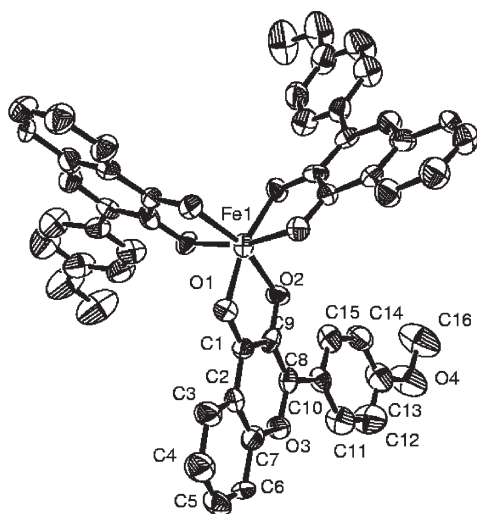
Fig. 2 The molecular structure of one of the two independent co-crystallized molecules of 2 with selected bond distances (Å) and angles (°): Fe1–O1 2.109(8), Fe1–O2 1.955(7), O1–C1 1.306(12), O2–C9 1.299(13), O3–C7 1.302(13), O3–C8 1.373(13), C1–C9 1.367(14), C1–C2 1.490(15), C2–C7 1.454(16), C8–C9 1.404(15); O2–Fe1–O1 80.0(3), O1–C1–C9 120.1(9). Ellipsoids are shown at the 50% probability level.
