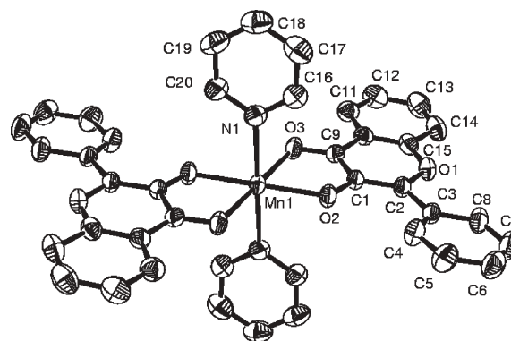
Fig. 1 The molecular structure of 1 with selected bond distances (Å) and angles (°): Mn1–O2 2.1274(16), Mn1–O3 2.1839(18), Mn1–N1 2.348 (2), O1–C15 1.351(3), O1–C2 1.374(3), O2–C1 1.302(3), O3–C9 1.257(3), C1–C9 1.460(3), C1–C2 1.385(3), C10–C15 1.393(3), C9–C10 1.437(4); O2–Mn1–O3 76.81(6), O2–Mn1–N1 90.99(7), N1–Mn1–N1* 180.0. *Symmetry code: (1 – x, 1 – y, 1 – z). Ellipsoids are shown at the 50% probability level.
