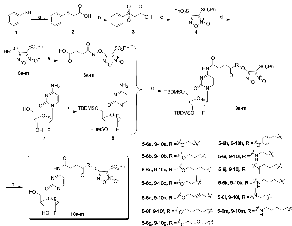
Scheme 1. Reaction conditions and reagents: a) 30 % NaOH, chloroacetic acid, Na 2 CO 3 , reflux, 1h, 89.0 %; b, c) HOAc, 30% H 2 O 2 , rt, 2.5h, 95 % HNO 3 , 90 °C, 0.5h, 76.0 %; d) diols or alcohol amines, 25 % NaOH or NaH, 0 °C, 0.5 h, 50.0-70.0 %; e) Succinic anhydride, CH 2 Cl 2 , reflux, 3-8 h, 85.0-92.7 %; f) TBDMSCl, imidazole, DMF, rt, 6 h, 87.3 %; g) NHS, EDCI, DMAP, rt, 18 h, 47.8-59.0 %; h) TBAF, THF, 0 °C, 0.5 h, 66.9-87.2 %.
