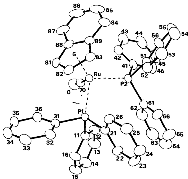
Fig. 2. A view of the cation [\text{Ru}(\text{CO})(\text{PPh}_3)_2(\eta^5\text{-C}_9\text{H}_7)]^+ , showing the coordination and the numbering system. The symbols of the carbon atoms are omitted for clarity.
