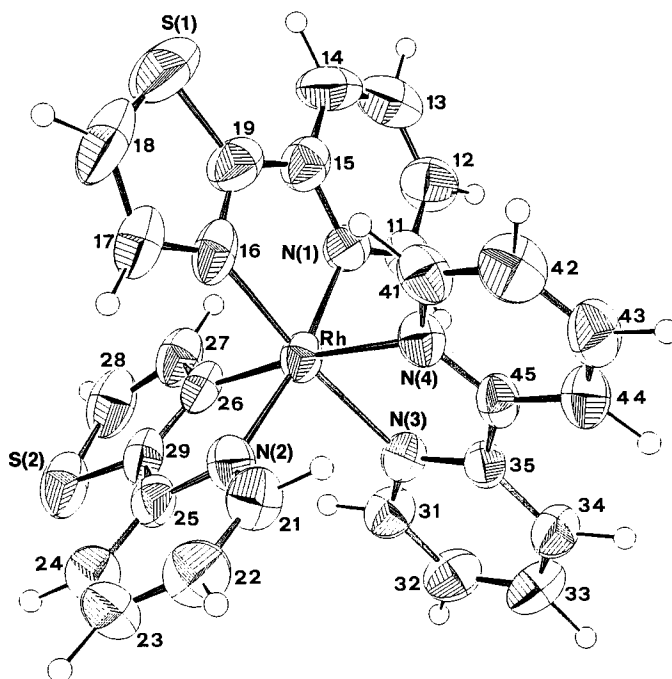
Fig. 1. ORTEP-II [30] diagram of the cation (2,2' -bipyridine) \text{bis}[2 -(thien-2-yl)pyridinato- \text{N},\text{C}^3 ]rhodium(III), showing the atomic-numbering (arbitrary) and the vibrational ellipsoids (50% probability level)
