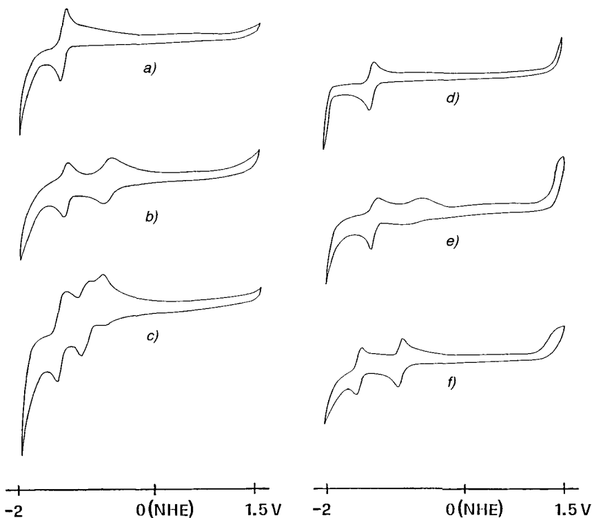
Fig. 3. Cyclic voltammograms of a) [\text{Rh}(2\text{-thpy})_2(\text{bpy})]^+ , b) [\text{Rh}(2\text{-thpy})_2(\text{phen})]^+ , c) [\text{Rh}(2\text{-thpy})_2(\text{biq})]^+ , d) [\text{Rh}(\text{ppz})_2(\text{bpy})]^+ , e) [\text{Rh}(3\text{-Clppz})_2(\text{bpy})]^+ , and f) [\text{Rh}(4\text{-NO}_2\text{ppz})_2(\text{bpy})]^+
