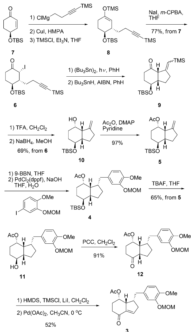
Scheme 2. Total Synthesis of Otteliones A and B
