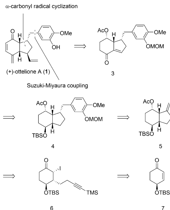
Scheme 1. Retrosynthetic Analysis of (+)-Ottelione A
