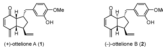
Figure 1. Structures of otteliones A and B.
