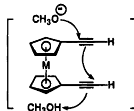
Figure 1. Methoxide attack and cyclization to [4]metallocenophanes.
