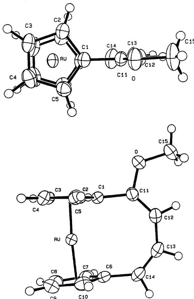
Figure 3. Top (above) and side (below) ORTEP views of 3b with crystallographic numbering scheme. Non-hydrogen atoms are represented as 50% probability thermal ellipsoids. Hydrogen atoms are drawn with an artificial radius.
