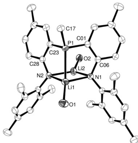
Figure 1. ORTEP drawing of the solid-state structure of 1 ·2THF (ellipsoids drawn at the 50% probability level). All hydrogen atoms and carbon atoms of THF and phenyl (except ipso C) have been omitted for clarity. Selected bond lengths (Å) and angles (deg): P1–Li1 2.510(3), N1–Li1 2.078(3), N1–Li2 2.046(4), Li1...Li2 2.518(4), O1–Li1 1.908(3), O2–Li2 1.932(3), N2–Li2 2.051(3), N2–Li1 2.076(3), P1–Li1–Li2 77.01(11), N1–Li2–N2 105.76(15), O1–Li1–Li2 144.07(18), C06–N1–C08 116.60(14), C01–P1–C23 105.40(8), C23–P1–C17 103.18(8), C01–P1–C17 105.62(8).
