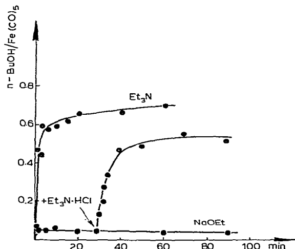
Fig. 7. Stoichiometric hydrogenation of n-butyraldehyde with \text{H}_2\text{Fe}(\text{CO})_4 in ethanol solution in the presence of \text{Et}_3\text{N} or \text{NaOEt} . Effect of added \text{Et}_3\text{NH} \cdot \text{HCl} .
