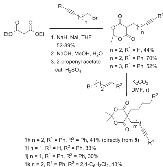
Scheme 3. Preparation of Alkenyl/Alkynyl Cascade Substrates
