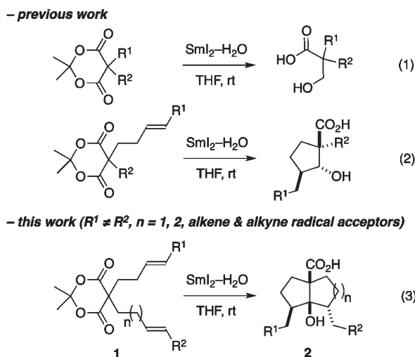
Scheme 1. Cyclization Cascades of Meldrum's Acid Derivatives
