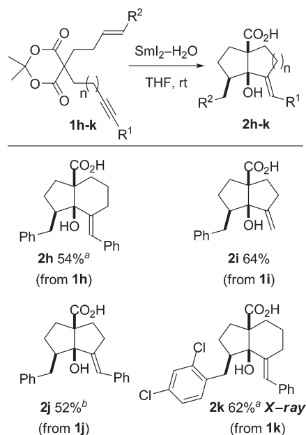
Figure 3. Cyclization Cascades Exploiting Alkene and Alkyne Radical Acceptors.
