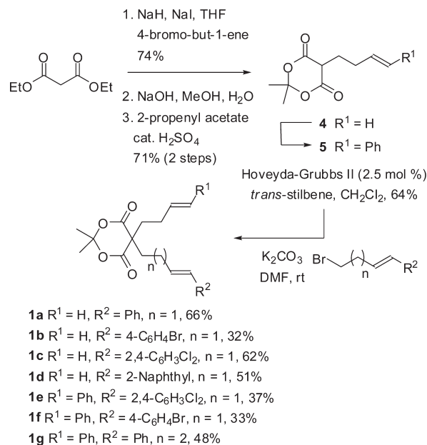
Scheme 2. Preparation of Alkenyl/Alkynyl Cascade Substrates
