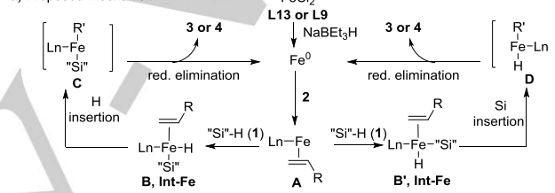
b) Proposed potential intermediates in the presence of tridentate ligand L13
