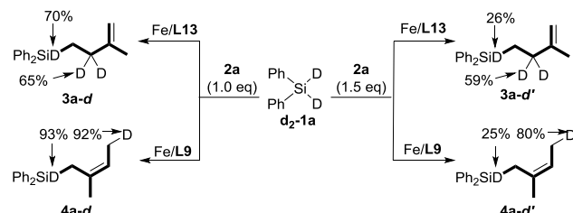
b) Deuterium labeling recovery experiments:
