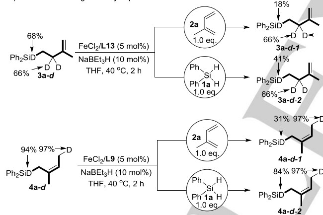
Scheme 4. Deuterium labeling studies.
