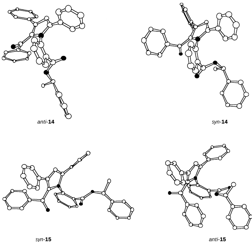
FIG. 2 Conformers of amides 14 and 15 optimised by the PM3 method (see text)
