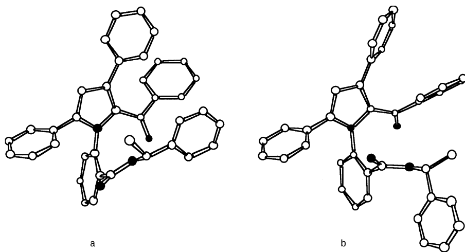
FIG. 3 Comparison of the X-ray molecular skeleton of amide 14 (a) with that obtained for anti -conformer of the compound calculated by the PM3 method (b)
