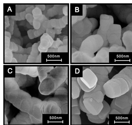
Fig. 2 SEM images of nano-sized TS-1 ns from microwave-assisted synthesis with different irradiation times of 10 min (A, TS-1 ns10 ), 20 min (B, TS-1 ns20 ), 60 min (C, TS-1 ns60 ) and 70 min (D, TS-1 ns70 ).
