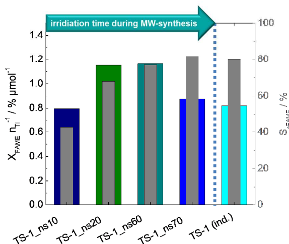
Fig. 11 Catalyst efficiency (conversion related to the amount of Ti atoms in the catalysts) for the epoxidation of biodiesel (FAME) with \text{H}_2\text{O}_2 over as well as epoxide selectivity ( S_{\text{eFAME}} ) over nano-sized TS-1 and conventional TS-1(ind.) after 5 h of reaction ( V_{\text{acetonitrile}} = 10 \text{ cm}^3 , c_{\text{FAME}} = 0.03 \text{ mol l}^{-1} , (n_{\text{H}_2\text{O}_2}/n_{\text{FAME}}) = 5 \text{ mol mol}^{-1} , m_{\text{cat.}} = 150 \text{ mg} , T = 323 \text{ K} ).
