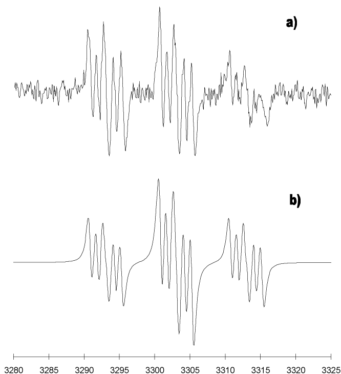
Figure 2. Epr spectra of radical anion 9 or 10 in dimethylsulphoxide, (a) experimental, (b) simulated. H.f.c.cs: a_H(C4)=10.03 ; a_H(C6)=9.85 ; a_H(C5)=2.45 ; a_{N-exo}=0.99 Gauss.
