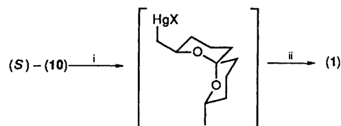
Scheme 3. Reagents and conditions: i, Hg(II) , H_2O -THF, H^+ , 18 h; ii, NaBH_4 , OH^- , CH_2Cl_2 , PTC.
