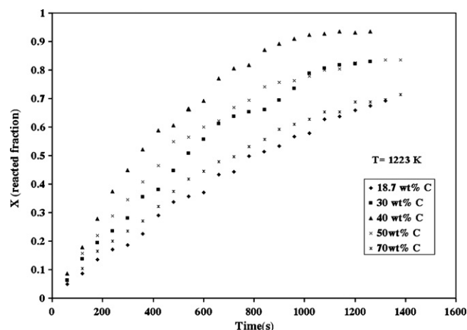
Fig. 4. Changes of reacted fraction versus reacting time at 1223 K, a gas flow rate of 400 l h -1 and a chlorine partial pressure of 0.3 atm.
