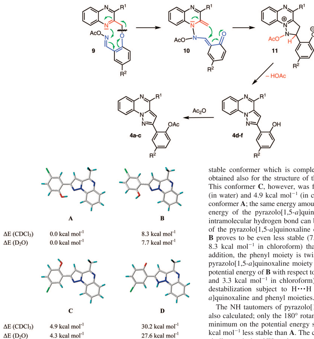
FIGURE 1. Structures of the pyrazolo[1,5- a ]quinoxaline derivative 4e [global minimum (A), without H-bonding (B), 180° rotamer (C), and NH tautomer (D)].
