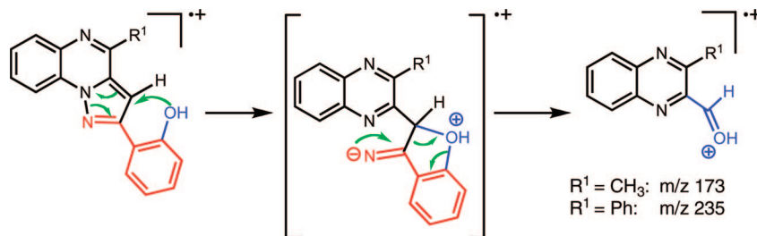
SCHEME 5. Fragmentation of the Pyrazolo[1,5- a ]quinoxaline Derivatives 4d–f
