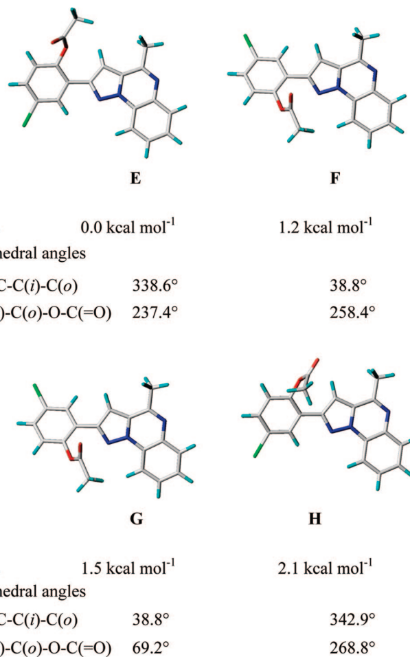
FIGURE 3. Structures of the pyrazolo[1,5- a ]quinoxaline derivative 4b [global minimum ( E ) and local minima structures ( F–H ); dihedral angles for the twist of the phenyl substituent ( N-C-C(i)-C(o) ) and of the OCOCH_3 moiety ( C(i)-C(o)-O-C(=O) ) are given ( i ipso; o ortho).
