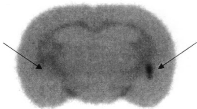
Figure 3. Autoradiographic image at 180 min post i.v. administration of 70 MBq of [ ^{18}\text{F} ]BF-168 in rat brain slice injected with \text{A}\beta(1\text{--}42) dissolved in phosphate buffer (right arrow) and buffer only (left arrow)
