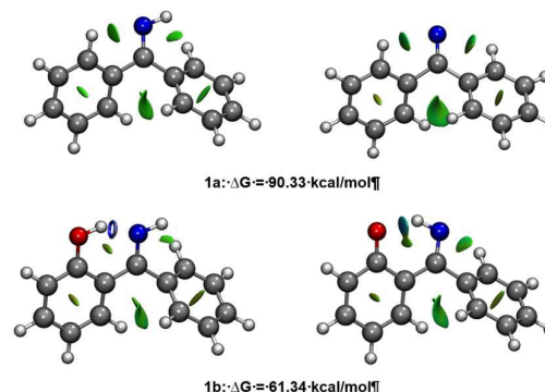
Figure 1. Gibbs free energies for deprotonated ketimine and ketimine 1a (top), and deprotonated hydroxylketimine and hydroxylketimine 1b (down). The gradient isosurfaces ( s = 0.5 a.u.) are coloured on a BGR scale according to the \text{sign}(\lambda_2)\rho over the range -0.05 to 0.05 a.u.
