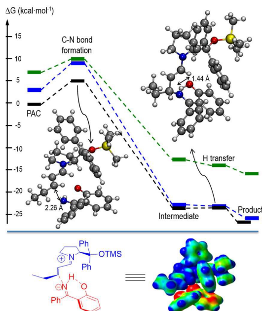
Figure 2. Gibbs free energy profile for the addition of ketimine 1b to aldehyde 2a catalysed by 3b . Three different orientations for the attack of 1b to the iminium are considered. The TSs for the C-N bond formation and H transfer in the lowest energy path are shown.
