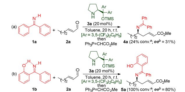
Scheme 2. Proof of concept in the reaction with ketimines 1a and 1b . a Determined by 1 H NMR. b Determined by chiral-SFC.
