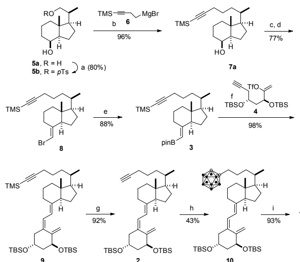
Scheme 2 Synthesis of target analog 1 . Reagents and conditions: a) pTSCl (1.5 equiv), py, 0 °C, 12 h; b) 6 (4 equiv), Et 2 O/THF (1:1); Li_2CuCl_4 (0.01 equiv), THF, -78 °C → 23 °C, 12 h; c) Oxidation of 7a to the corresponding ketone 7b : PDC (3 equiv), CH 2 Cl 2 , 23 °C, 5 h; d) (Ph_3PCH_2Br)Br (8 equiv), tol, ultrasound, 15 min; KOtBu in THF (7.9 equiv, 1 M), -15 °C → 0 °C, 2.5 h, then 7b in tol, -15 °C → 23 °C, 3 h; e) Tol/THF (3:1), -78 °C, tBuLi (2 equiv), 1 h; B(OiPr)_3 (1.5 equiv), 1.5 h; pinacol (1.3 equiv), -78 °C → 23 °C, 4 h; f) 4 (1 equiv), K_3PO_4 (27 equiv, aqueous sol, 2 M), THF, PdCl_2(PPh_3)_2 (0.05 equiv), 2 h; g) K_2CO_3 , MeOH, 23 °C, 14 h; h) PhNMe 2 (6.5 equiv), tol, decaborane ( B_{10}H_{14} , 3 equiv), 110 °C, 1 h; i) HF (48%, 2.5 equiv), CH 2 Cl 2 /CH 3 CN (2:1), 23
