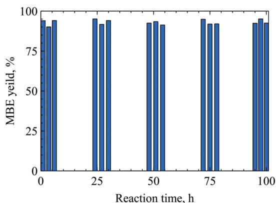
Fig. 9 Long-term stability of the capillary microreactor with Pd-Bi/TiO 2 in MBY semihydrogenation (1200 \text{mol m}^{-3} MBY in hexane flow 42.5 \mu\text{L min}^{-1} , 10 \text{mL min}^{-1} (STP) H 2 flow, 335 K).
