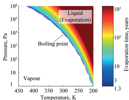
Fig. 1 Effect of temperature and pressure on the evaporation time of the 5 \text{ m} long reactor filled with ethanol, estimated using Stefan's equation. 33
