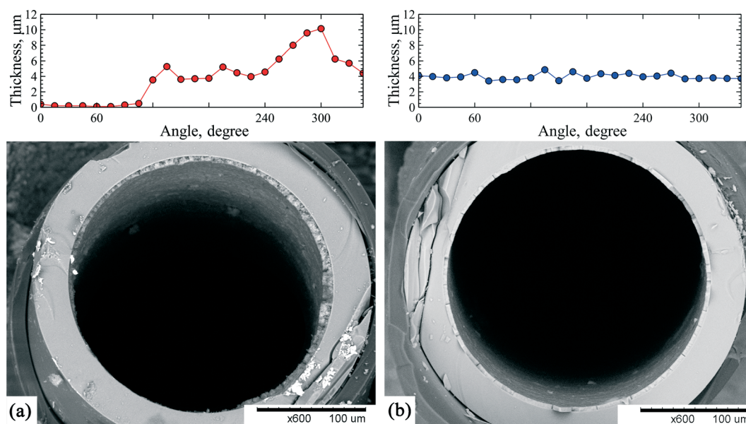
Fig. 5 Cross-sectional SEM images of the capillaries coated at (a) 0.2 mm s -1 , (b) 5 mm s -1 and the coating thickness as a function of angular position.
