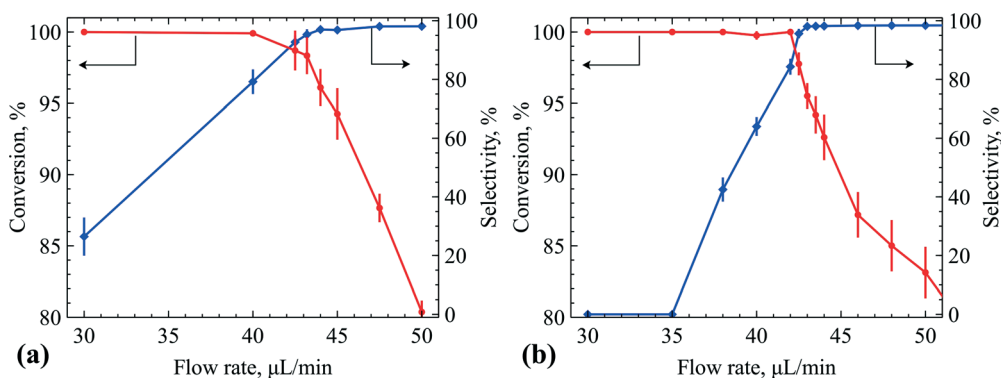
Fig. 8 Summary of the performance of the capillary microreactor with Pd–Bi/ \text{TiO}_2 in MBY semihydrogenation ( 1200\ \text{mol m}^{-3} MBY in hexane, 10\ \text{mL min}^{-1} (STP) \text{H}_2 flow, (a) 310\ \text{K} and (b) 335\ \text{K} ). Selectivity is calculated towards MBE.
