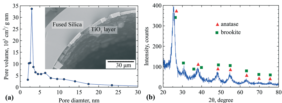
Fig. 4 (a) PSD of the TiO 2 coatings, (insert) SEM image of the cross-section of the titania coated 250 μm capillary, and (b) the PXRD pattern of the coating.
