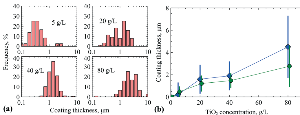
Fig. 6 (a) Distribution of the \text{TiO}_2 coating thickness obtained in the 250\ \mu\text{m} fused silica capillaries using different precursor sol concentrations. Displacement speed: 0.2\ \text{mm s}^{-1} . Oven temperature: 450\ \text{K} . (b) The comparison of the average coating thickness determined by (●) SEM and (◆) hydrodynamic study.
