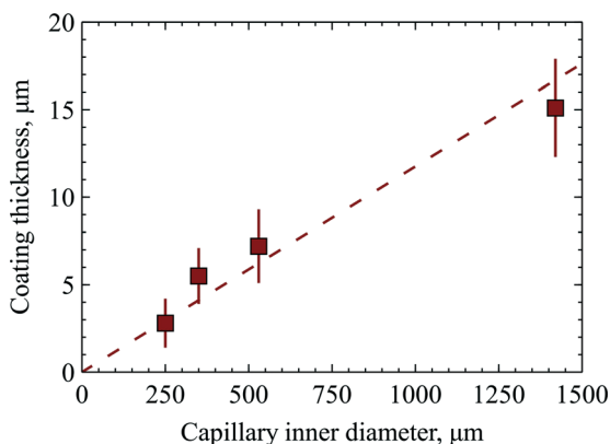
Fig. 7 Effect of the capillary inner diameter on the coating thickness (SEM data) using a 80\ \text{g L}^{-1} \text{TiO}_2 sol.
