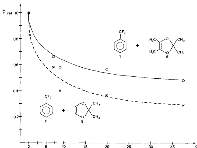
Fig. 1. Dependence of the quantum yields of product formation on solvent polarity in photoreactions of \alpha,\alpha,\alpha -trifluorotoluene (1) with tetramethyl- and 2,2-dimethyl-1,3-dioxole (6 and 8, resp.).
