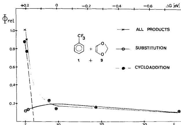
Fig. 2. Dependence of the product quantum yields or solvent polarity for both substitution and cycloaddition in the photoreaction of \alpha,\alpha,\alpha -trifluorotoluene 1 with 1,3-dioxole 9
