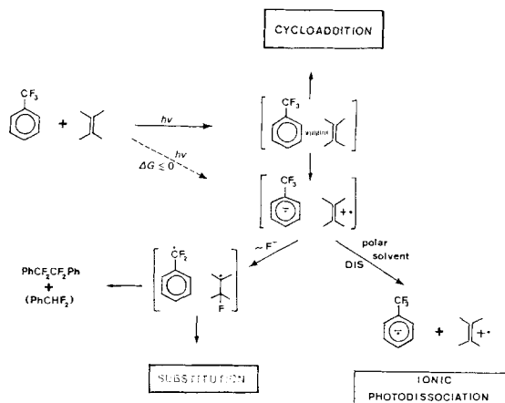
Scheme 2. Proposed Mechanism of Photoreactions of \alpha,\alpha,\alpha -Trifluorotoluene with Olefins
