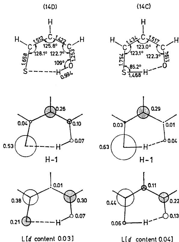
FIGURE 1 Calculated geometries (CNDO/B) and population analysis (CNDO/S-CI) of the H-1 and L levels in the enol and ethanion tautomers of monothiomalondialdehyde (14). Diameters of circles are proportional to the square of the contributing atomic orbital coefficients. U.v. (CNDO/S-CI): (14D), 339 nm [H-1, L (0.97), H-2, L + 1 (0.03)]; (14C), 304 nm [H-1, L (0.93), H, L + 2 (0.03), H, L + 3 (0.02), H-2, L + 1 (0.01)]
