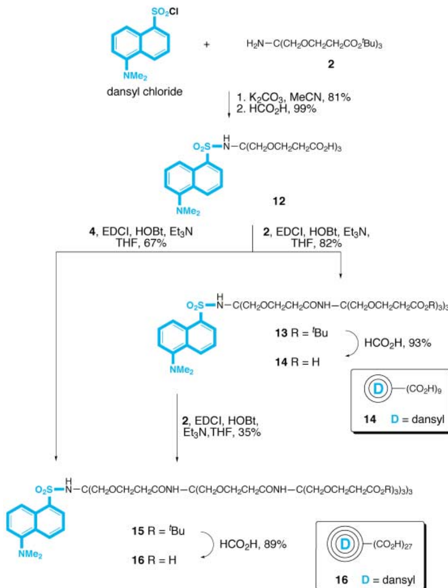
Scheme 3. Synthesis of G2 and G3 Dansyl Nona- and 27-Acid Dendrimers
