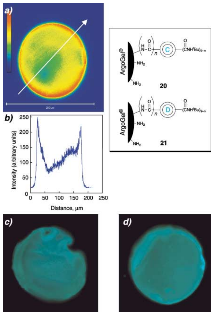
Fig. 10. a) LSCM Image of the center of G2 coumarin/dendrimer bead 20 . b) Intensity profile of emitted light along path of white arrow in a. c) EFM Image of a wafer, ca. 5-μm thick, of G2 coumarin/dendrimer bead 20 . d) EFM Image of a microtome wafer of G2 dansyl/dendrimer bead 21 .
