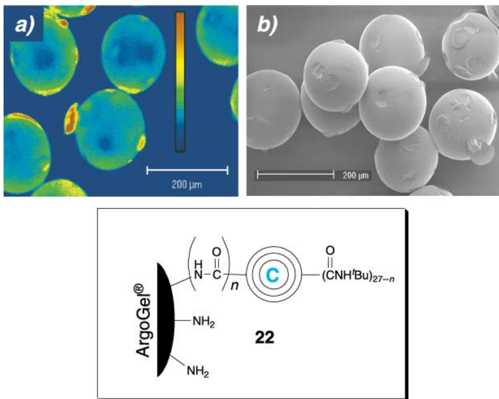
Fig. 7. a) LSCM Image ( 10\times objective) of a plane bisecting a group of G3 dendrimer beads 22 (false color shows relative intensity of emitted light: red is brightest). b) ESEM Image of 22 .
