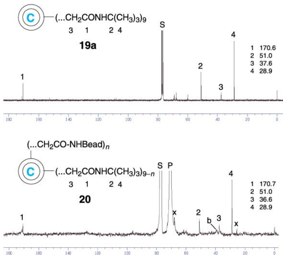
Fig. 6. a) ^{13}\text{C} -NMR Spectrum of 19a . S = \text{CDCl}_3 . b) ^{13}\text{C} -NMR Spectrum of ArgoGel® beads with G2 coumaryl dendrimer covalently attached; 20 (Scheme 5 and text). S = \text{CDCl}_3 ; b = minor signal from resin; P = \text{CH}_2\text{O} C-atoms of polyethylene glycol (PEG) grafts on the resin; x = THF.
