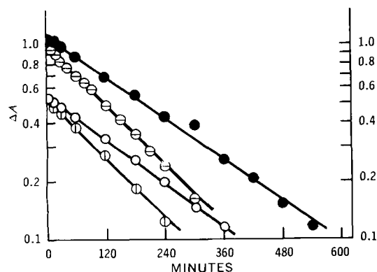
Figure 3 —Semilogarithmic plot of absorbance change versus time for epitetracycline (● at 356 nm and ○ at 427 nm) and tetracycline (⊙ at 356 nm and ⊖ at 433 nm) at 70° and pH 2.0.
