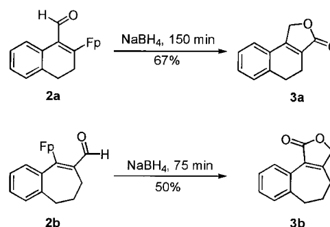
Scheme 2. \text{Fp} = [\eta^5\text{-C}_5\text{H}_5(\text{CO})_2\text{Fe}] .
