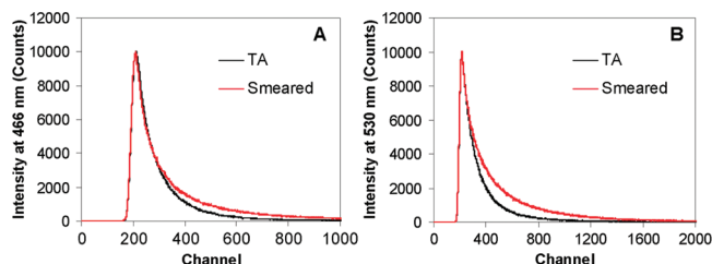
Figure 5. Fluorescence lifetime decays of a BF 2 dbmOC 12 H 25 (control) solid film on a piece of weighing paper monitored at 466 nm (A) and 530 nm (B) ( \lambda_{ex} = 369 nm LED). TA: thermally annealed.
