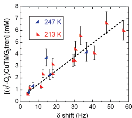
Figure 4. Determination of the solution magnetic moment of [\text{Cu}(\eta^1\text{-O}_2)\text{TMG}_3\text{tren}]^+ . Data at 213 K and 247 K are shown on one correlation line to illustrate the temperature insensitivity of \mu_{\text{eff}} .
