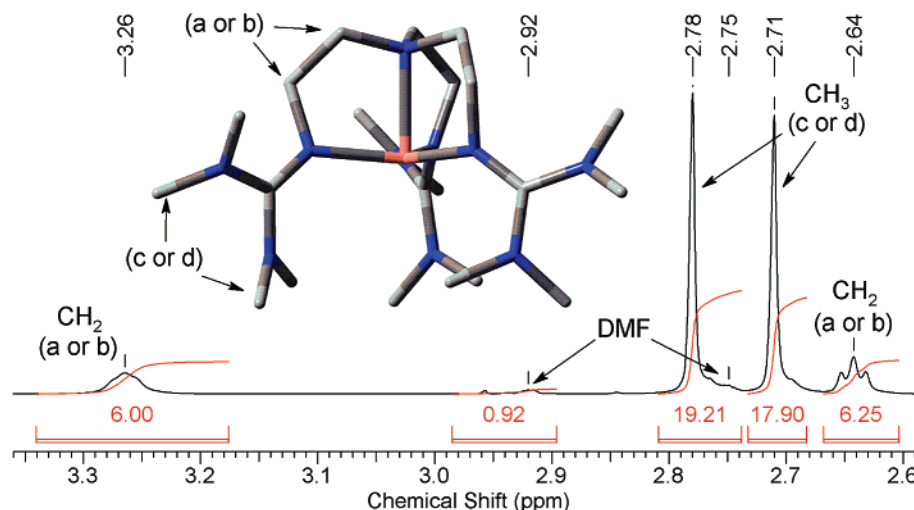
Figure 1. ^1\text{H} NMR spectrum (500 Mhz) of [\text{Cu}^{\text{I}}(\text{TMG}_3\text{tren})]^+ in \text{DMF-}d_7 at 298 K.
