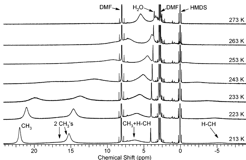
Figure 2. ^1\text{H} NMR spectra (300 MHz) revealing the increased concentration of [\text{Cu}(\eta^1\text{-O}_2)\text{TMG}_3\text{tren}]^+ in \text{O}_2 -saturated \text{DMF-}d_7 as the temperature is lowered from 273 to 213 K. The internal standard, hexamethyldisiloxane (HMDS) is noted. Only the region between 28 and -9 ppm is shown. Additional signals are observed at \sim 65 and 300 ppm.
