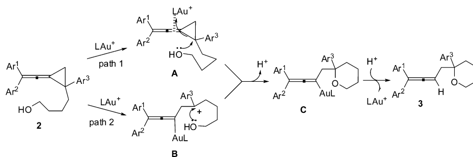
Scheme 3. Mechanisms of Au(I)-Catalyzed Intramolecular Addition/Ring-Opening of VDCPs
