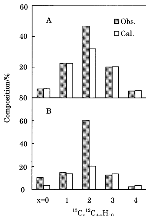
Figure 1. ^{13}\text{C} -Distributions of isobutane in the isomerization of 1,4- ^{13}\text{C}_2 - n -butane over \text{Cs}_{2.5}\text{H}_{0.5}\text{PW}_{12}\text{O}_{40} . A: 393 K (Conv. =10%) and B: 523 K (Conv. =11%).
