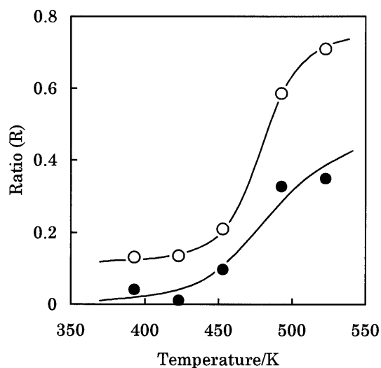
Figure 2. Ratio ( R ) of contribution of monomolecular pathway to that of bimolecular pathway. \text{Cs}_{2.5}\text{H}_{0.5}\text{PW}_{12}\text{O}_{40} ( \circ ) and \text{SO}_4^{2-}/\text{ZrO}_2 ( \bullet ). The conversions were around 10%.
