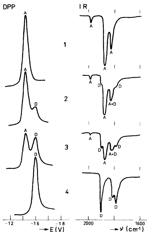
Fig. 1. Electrode-catalyzed preparation of W(CO)_3PPh_3bipy as monitored by dp-polarography and IR spectra in THF at T 291 K. (1) 0.01 M W(CO)_4bipy , 0.03 M PPh_3 ; (2) after partial reduction ( n_{app} 0.07 F mol^{-1} ); (3) solution 2 10 min after interruption of electrolysis; (4) complete conversion ( n 0.23 F mol^{-1} ). A, dp-peak and CO-bands of W(CO)_4bipy ; D, dp-peak and CO-bands of W(CO)_3PPh_3bipy .
