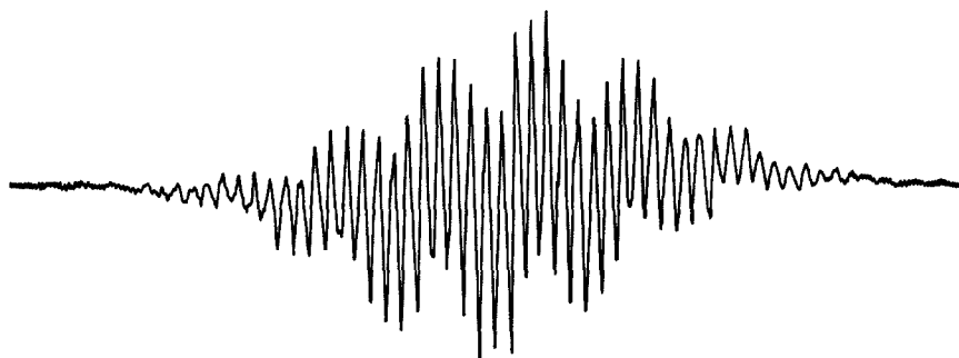
Fig. 3. EPR spectrum of \text{Mo(CO)}_4\text{bipy}^- in THF at 291 K ( g = 2.004 ; hyperfine coupling constants (mT): a_N = 0.35 ; a_H = 0.12 ; 0.10 ; 0.42 ; 0.07 ; a_{\text{Mo}} = 0.16 )
