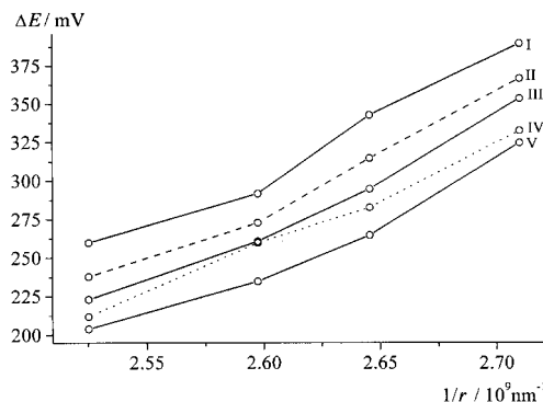
Figure 9. \Delta E versus 1/r for the [\text{M}(\text{FcCyclam})](\text{CF}_3\text{SO}_3)_2 complexes ( \text{M}^{2+} = \text{Zn}^{2+} , \text{Cu}^{2+} , \text{Ni}^{2+} , and \text{Co}^{2+} ) in \text{CH}_3\text{CN}/\text{THF} mixtures (I 30:10; II 30:20; III 30:30; IV 20:30; V 10:30).
