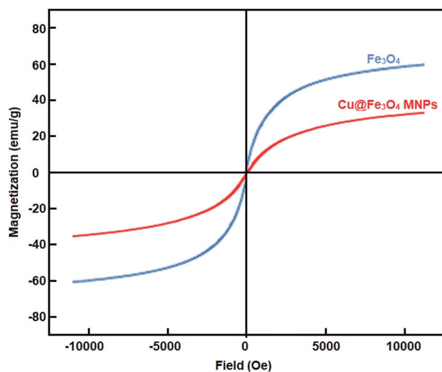
Fig. 3 VSM magnetization curves corresponding to the bare \text{Fe}_3\text{O}_4 and \text{Cu@Fe}_3\text{O}_4 MNPs.
