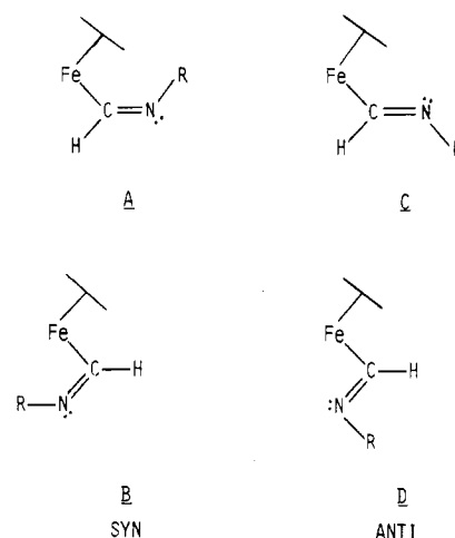
Figure 1. Four possible isomers of \text{Cp}(\text{CO})_2\text{Fe}(\text{CH}=\text{NR}) (CO groups omitted for clarity).
